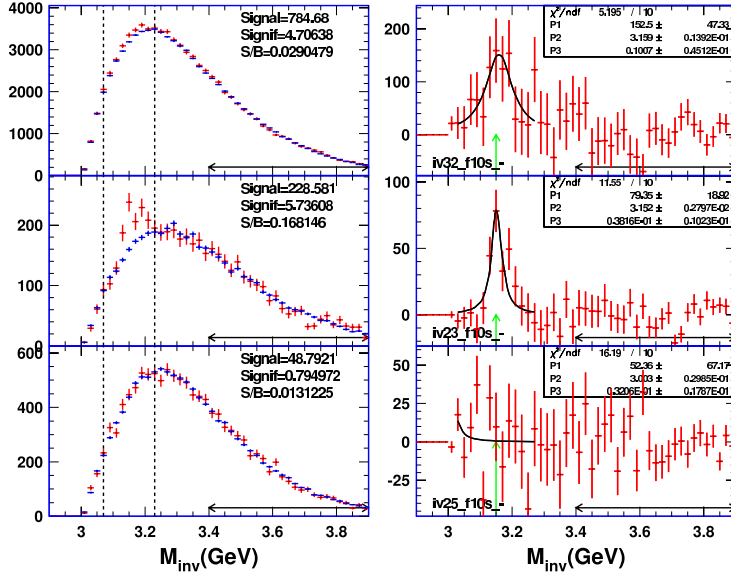
Figure 5: Invariant mass distributions of \Lambda -d pairs. On the left side combinatorial (red) and mixed event (blue) distributions are shown. They are normalized to each other within the range indicated by the horizontal arrow shown in the subpanels. The statistical information is evaluated in the interval defined by the vertical dashed lines.
