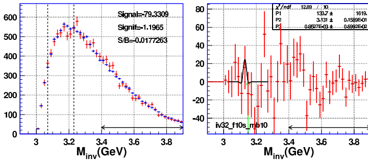
Figure 6: Invariant mass distributions of \Lambda -background - d pairs. Pairs of p\pi^- tracks fulfilling the \Lambda -selection criteria with 10 \text{ MeV} < |M_{inv} - 1116 \text{ MeV}| < 20 \text{ MeV} are combined with d-tracks. The layout of the figure is the same as in Fig. 5. Further details are described in the text.
