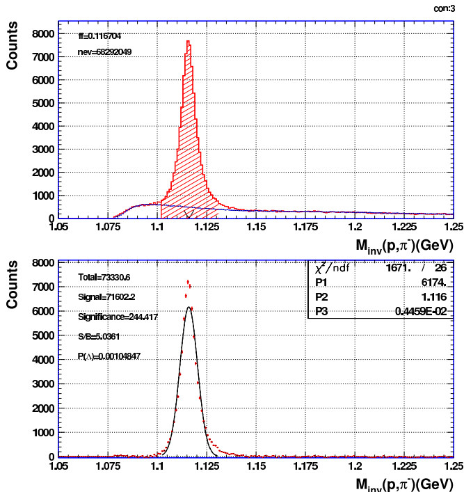
Figure 2: Invariant mass distribution of proton- \pi^- pairs under the selection criteria used for the ppnK^- analysis
