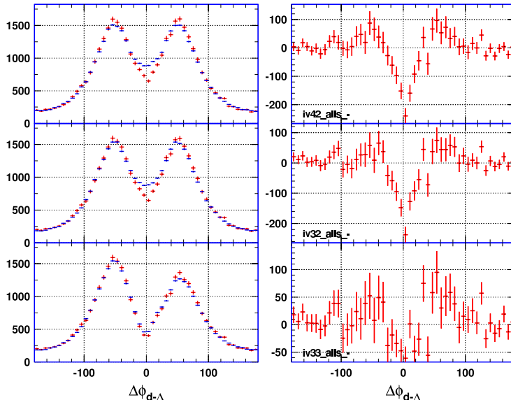
Figure 4: Difference of azimuthal angle distribution of \Lambda candidates and deuterons. The layout and conditions are the same as for Fig. 3.
