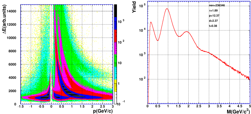
Figure 1: Correlation of the specific energy loss in the central drift chamber with the particle momentum determined from the track curvature (left). On the right side the mass distribution derived from linearizing the distribution with a Bethe-Bloch parametrisation for particles with a charge Z=1 is shown.
