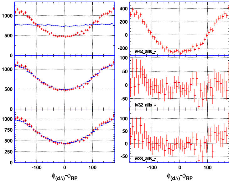
Figure 3: Azimuthal distribution of \Lambda candidates - deuteron pairs with respect to the reaction plane under different correlation criteria. In the left column correlated (mixed) pairs are shown by red (blue) crosses. In the right column the difference is plotted. For further details see text.
